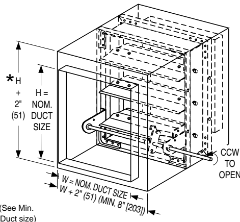
STYLE CSR : FOR SQUARE OR RECTANGULAR DUCT
