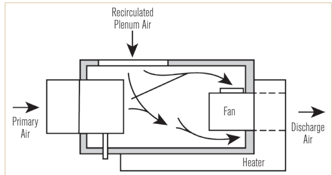
FIGURE 4 Series fan box.
