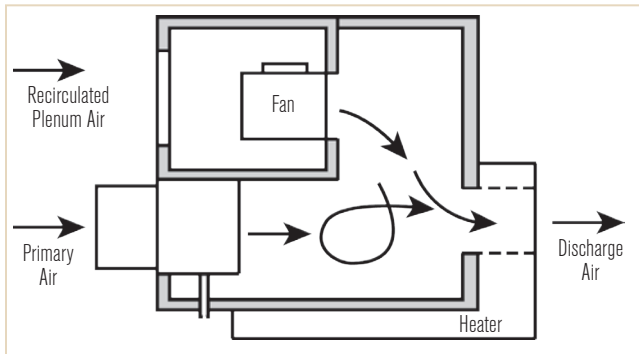
FIGURE 3 Parallel fan box.
