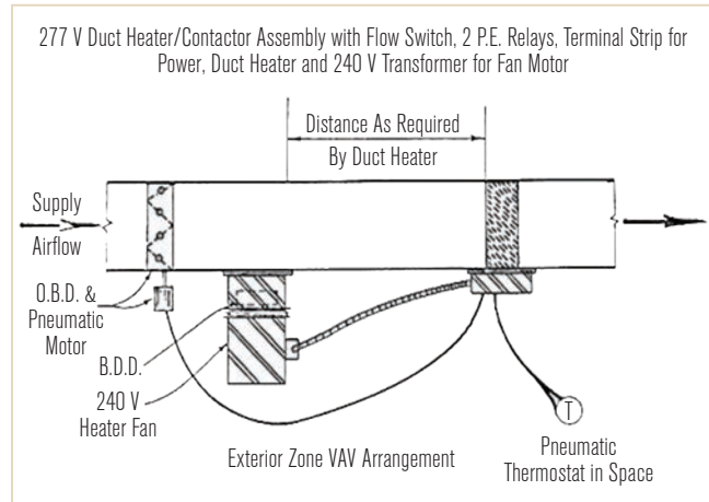
FIGURE 2 Early parallel box layout.
