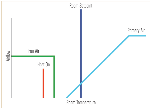
FIGURE 1 Parallel box control sequence.
