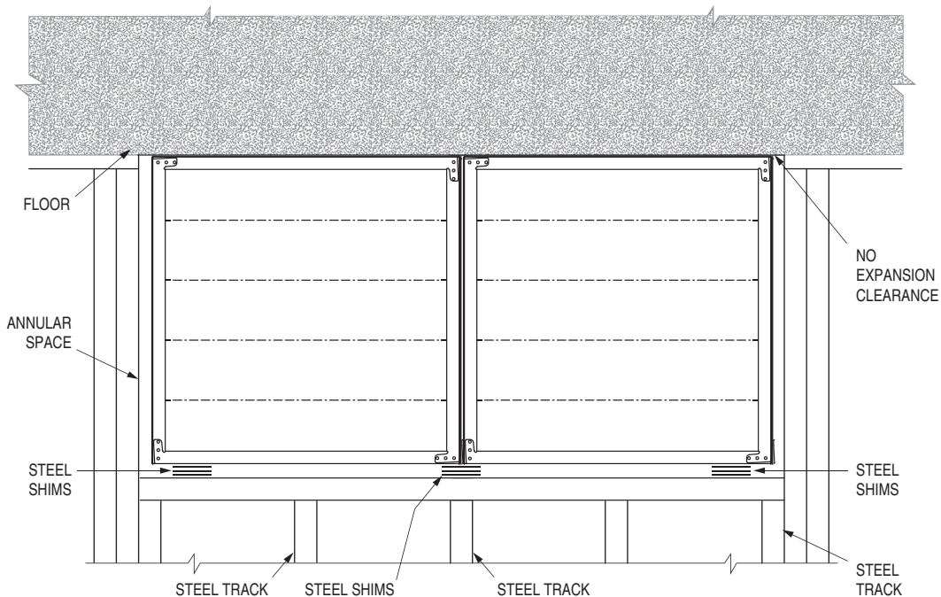
Figure 4: Steel shims installed and left underneath multi-section damper to push tight up against the above surface.
