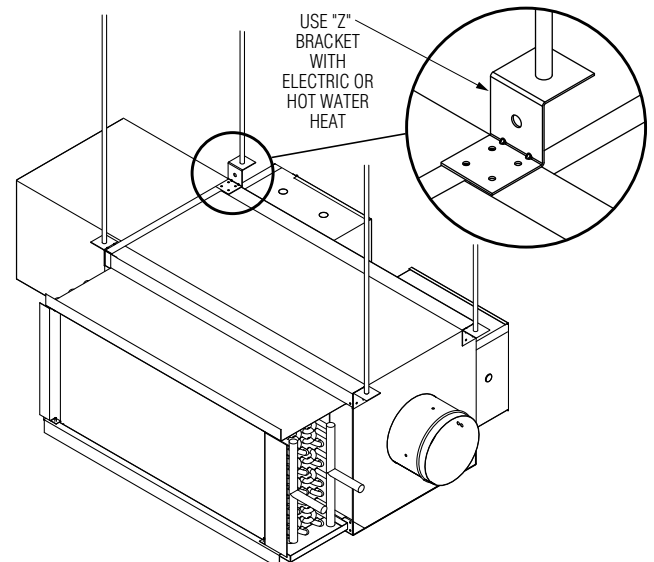
Figure 2: Fan Powered Chilled Water Terminal Unit Support Using Hanger Brackets and Rods (Model 33SZ unit size 40/50/55 illustrated).
