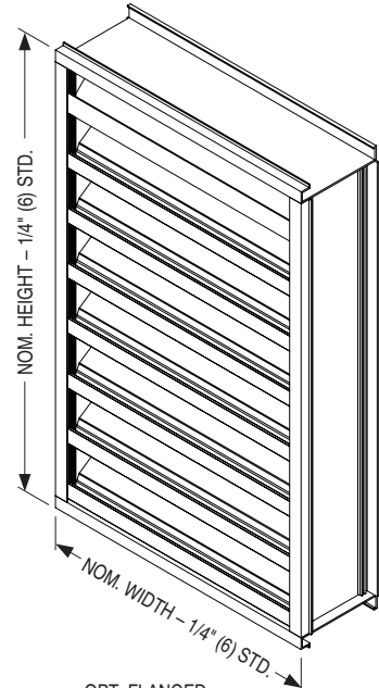
OPT. FLANGED FRAME (FL15 STD.) 1 1/2" (38)
