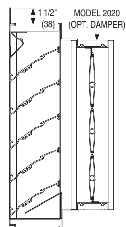
OPT. FLANGED FRAME (FL15 STD.) 1 1/2" (38)
